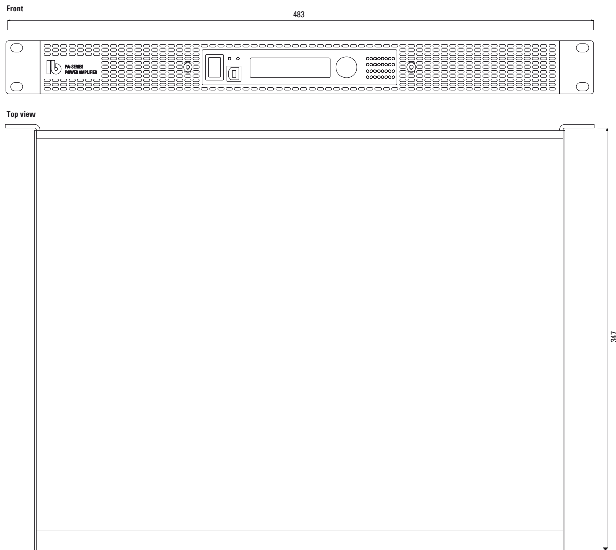
PA 4100/4200/4400 DSC
