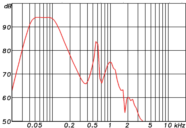
Frequency response B 212 B 1W/1m (full space)
